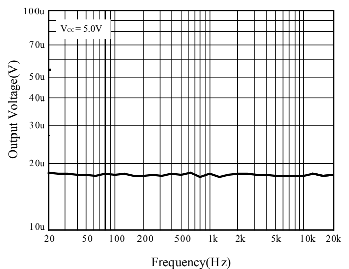
Figure 8 Noise Floor
